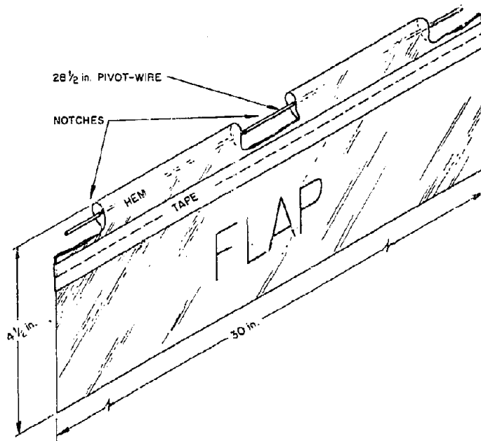
Fig. B-7. Finished flap.
